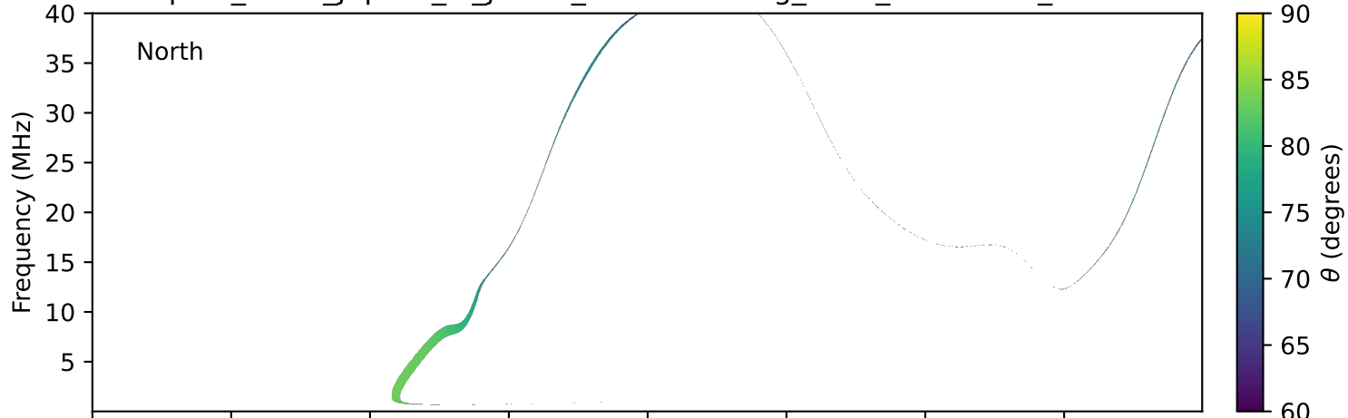
expres_earth_jupiter_io_jrm33_lossc-wid1deg_3kev_20140108_v11.cdf
