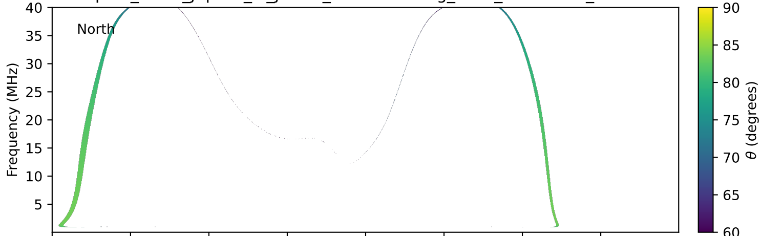
expres_earth_jupiter_io_jrm33_lossc-wid1deg_3kev_20140103_v11.cdf
