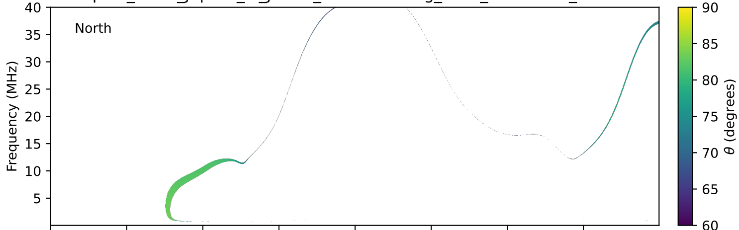
expres_earth_jupiter_io_jrm33_lossc-wid1deg_3kev_20140101_v11.cdf
