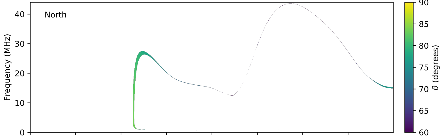
expres_earth_jupiter_io_jrm09_lossc-wid1deg_3kev_20140131_v01.cdf
