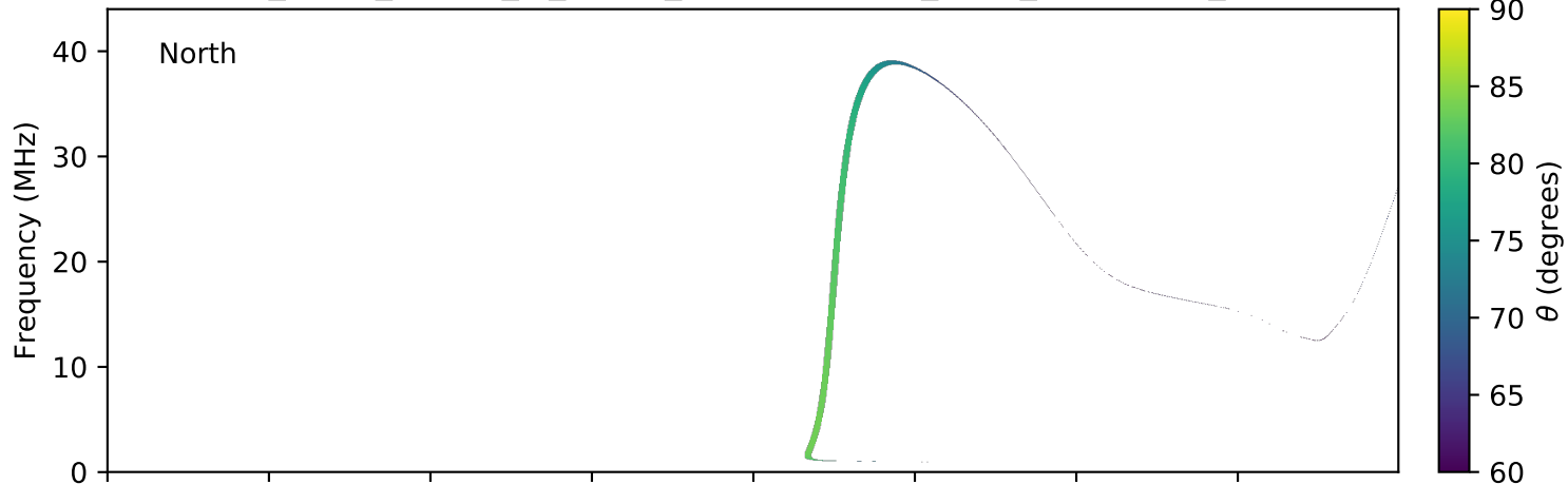
expres_earth_jupiter_io_jrm09_lossc-wid1deg_3kev_20140129_v01.cdf
