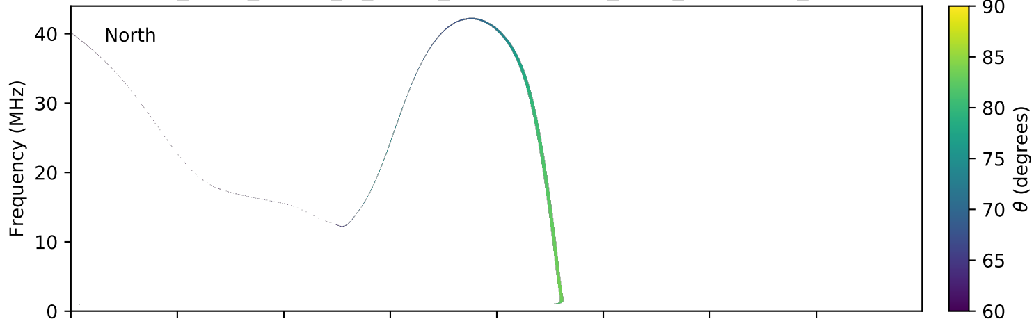
expres_earth_jupiter_io_jrm09_lossc-wid1deg_3kev_20140128_v01.cdf
