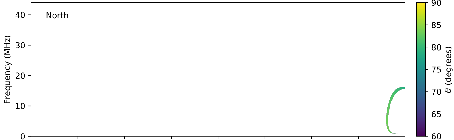
expres_earth_jupiter_io_jrm09_lossc-wid1deg_3kev_20140125_v01.cdf
