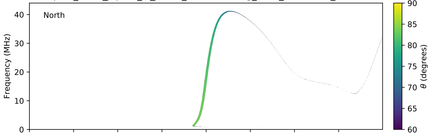
expres_earth_jupiter_io_jrm09_lossc-wid1deg_3kev_20140122_v01.cdf
