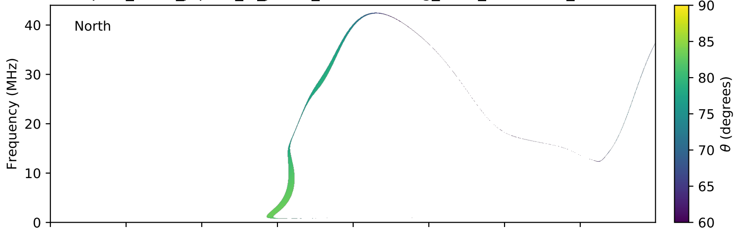
expres_earth_jupiter_io_jrm09_lossc-wid1deg_3kev_20140115_v01.cdf
