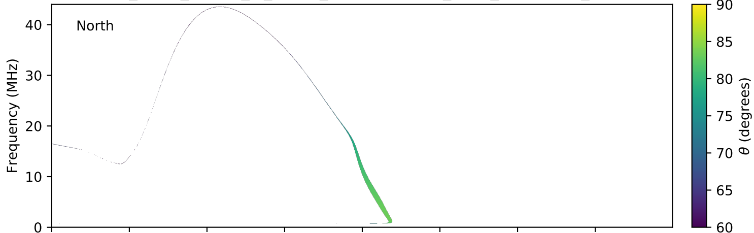
expres_earth_jupiter_io_jrm09_lossc-wid1deg_3kev_20140105_v01.cdf
