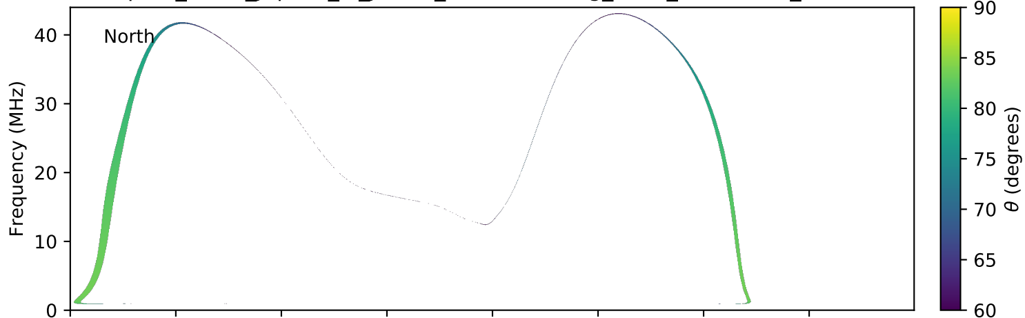
expres_earth_jupiter_io_jrm09_lossc-wid1deg_3kev_20140103_v01.cdf
