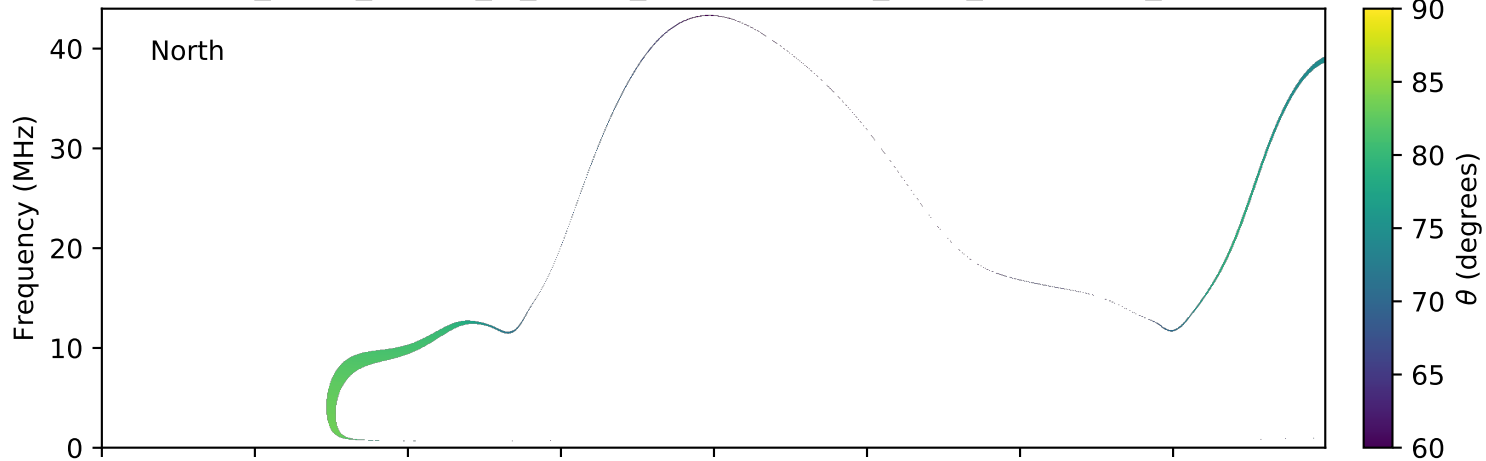
expres_earth_jupiter_io_jrm09_lossc-wid1deg_3kev_20140101_v01.cdf
