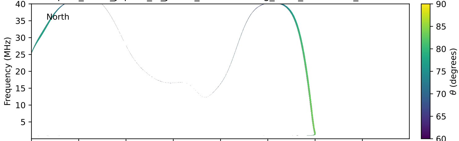
expres_earth_jupiter_io_jrm33_lossc-wid1deg_3kev_20131227_v11.cdf
