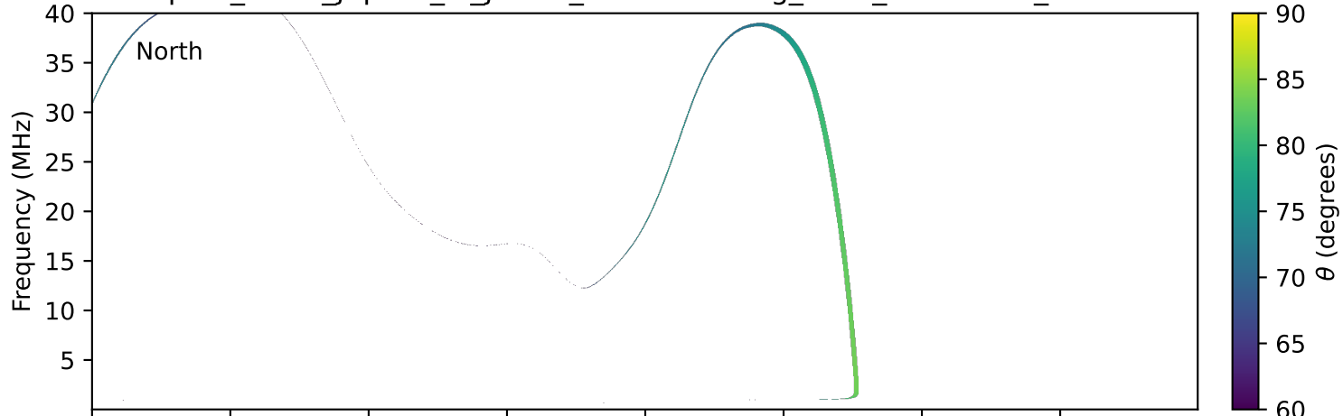
expres_earth_jupiter_io_jrm33_lossc-wid1deg_3kev_20131220_v11.cdf
