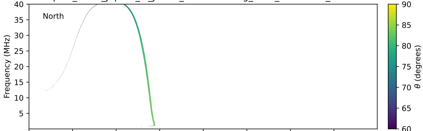
expres_earth_jupiter_io_jrm33_lossc-wid1deg_3kev_20131215_v11.cdf
