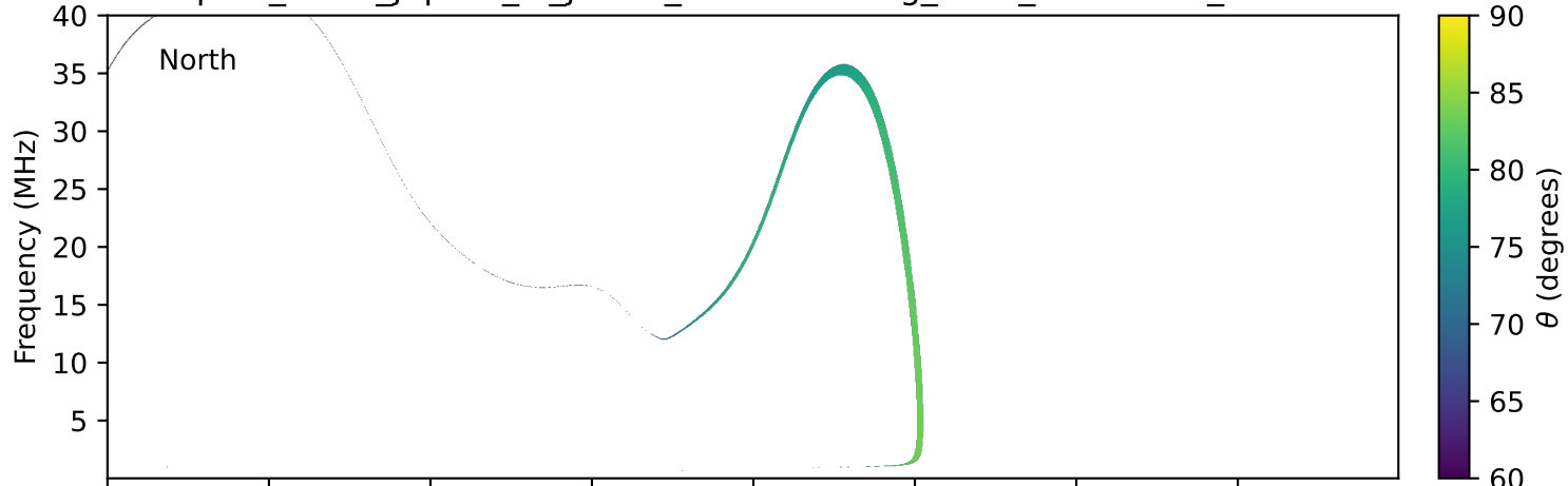
expres_earth_jupiter_io_jrm33_lossc-wid1deg_3kev_20131213_v11.cdf
