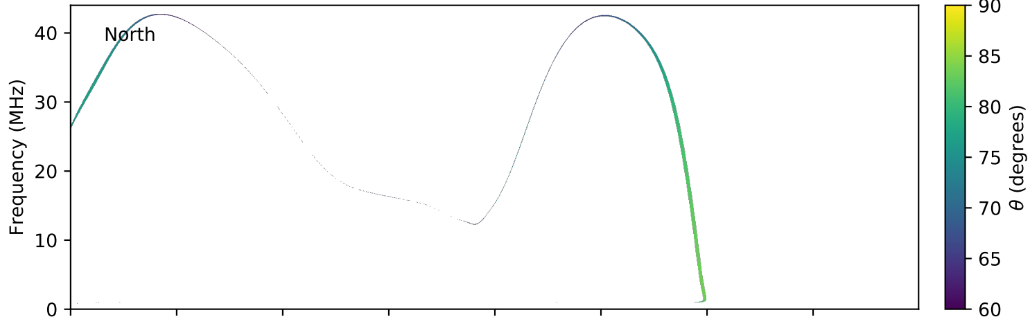
expres_earth_jupiter_io_jrm09_lossc-wid1deg_3kev_20131227_v01.cdf
