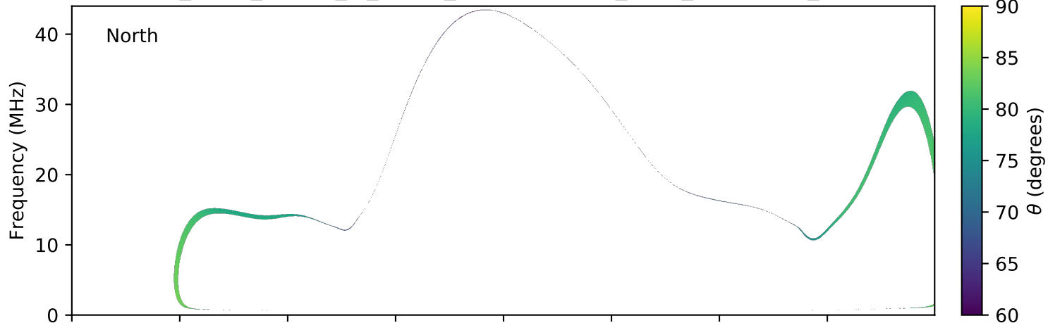
expres_earth_jupiter_io_jrm09_lossc-wid1deg_3kev_20131225_v01.cdf
