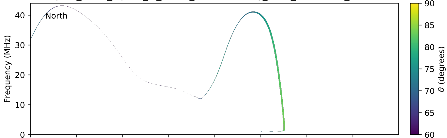
expres_earth_jupiter_io_jrm09_lossc-wid1deg_3kev_20131220_v01.cdf
