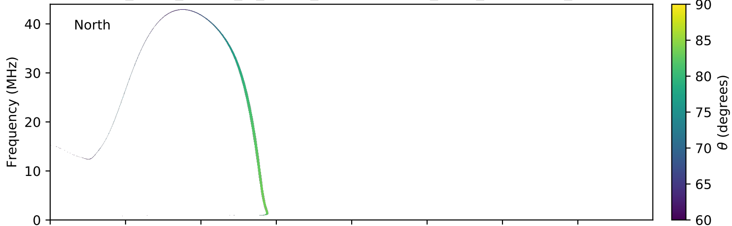
expres_earth_jupiter_io_jrm09_lossc-wid1deg_3kev_20131215_v01.cdf
