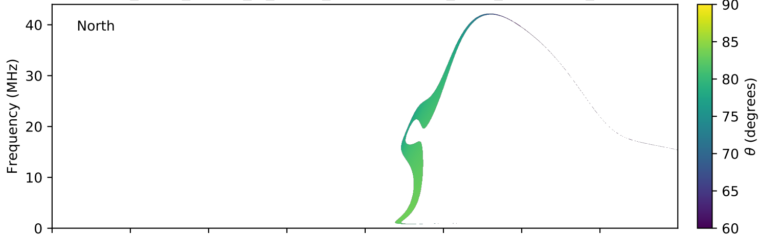
expres_earth_jupiter_io_jrm09_lossc-wid1deg_3kev_20131214_v01.cdf
