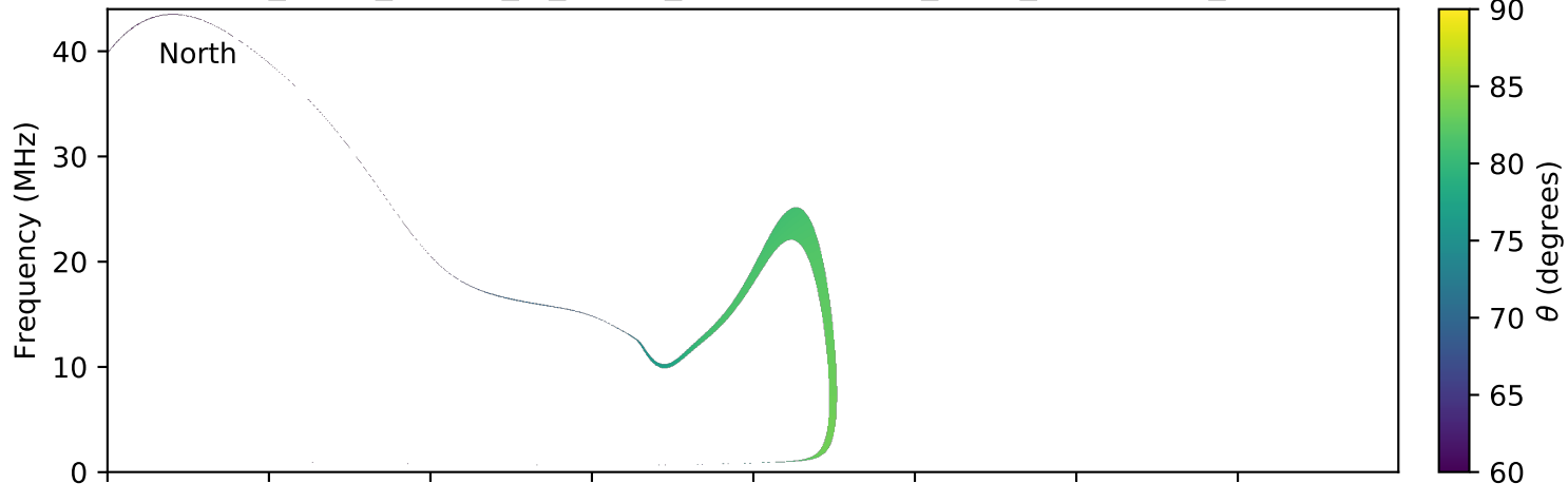
expres_earth_jupiter_io_jrm09_lossc-wid1deg_3kev_20131206_v01.cdf
