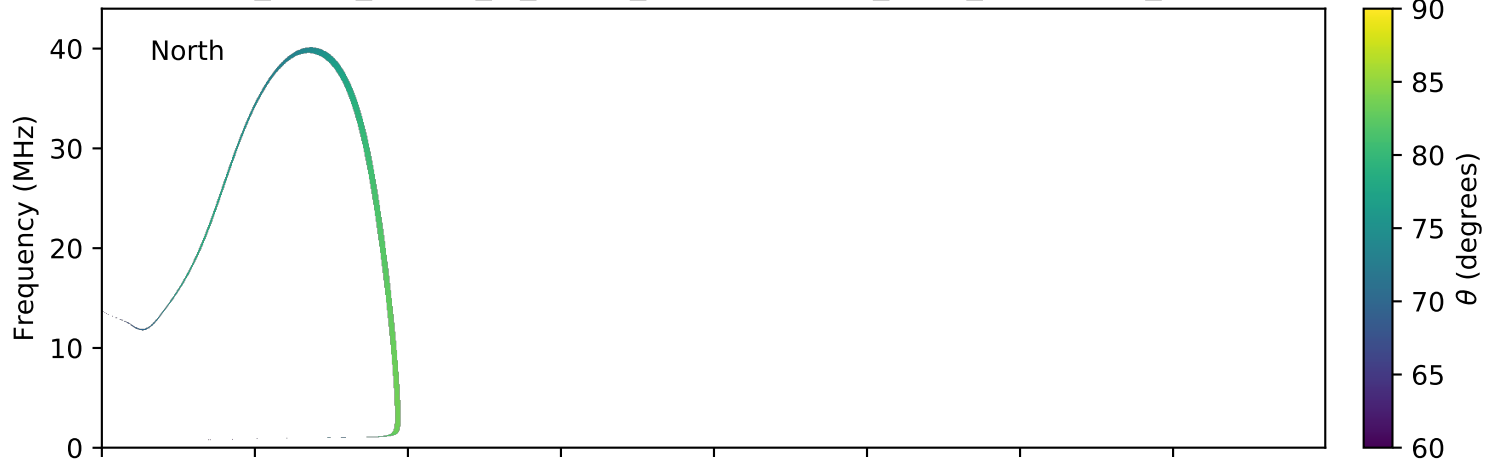
expres_earth_jupiter_io_jrm09_lossc-wid1deg_3kev_20131201_v01.cdf
