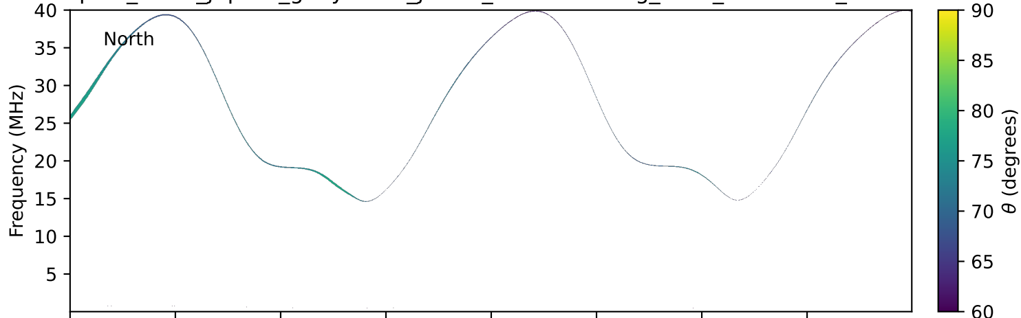
expres_earth_jupiter_ganymede_jrm33_lossc-wid1deg_3kev_20131220_v11.cdf
