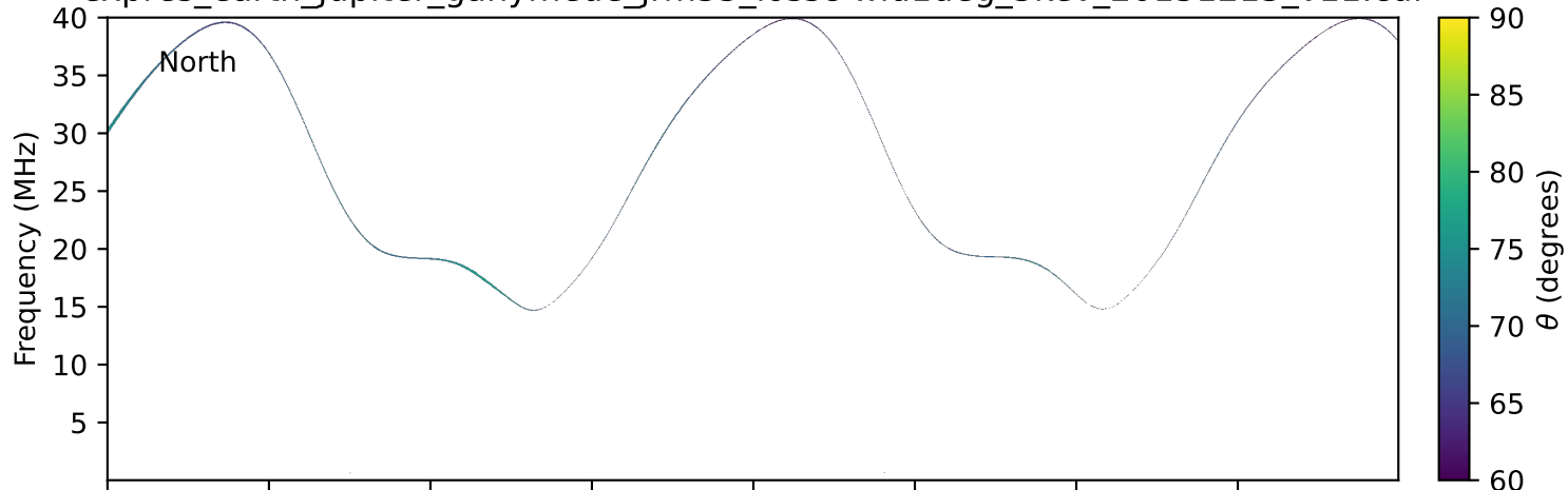
expres_earth_jupiter_ganymede_jrm33_lossc-wid1deg_3kev_20131213_v11.cdf
