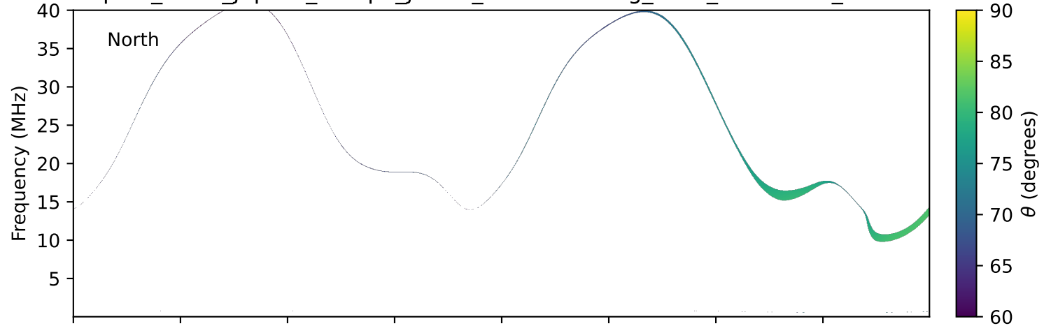
expres_earth_jupiter_europa_jrm33_lossc-wid1deg_3kev_20131215_v11.cdf
