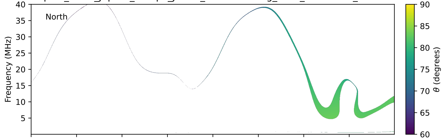
expres_earth_jupiter_europa_jrm33_lossc-wid1deg_3kev_20131208_v11.cdf
