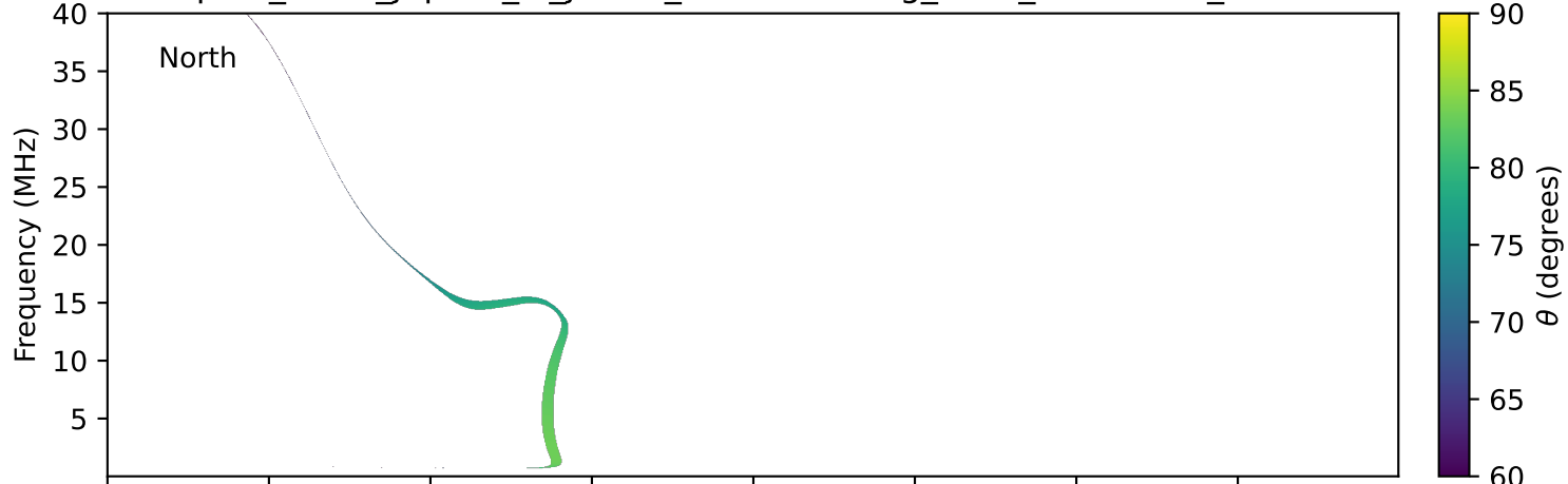
expres_earth_jupiter_io_jrm33_lossc-wid1deg_3kev_20131122_v11.cdf
