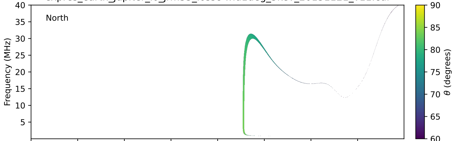
expres_earth_jupiter_io_jrm33_lossc-wid1deg_3kev_20131121_v11.cdf
