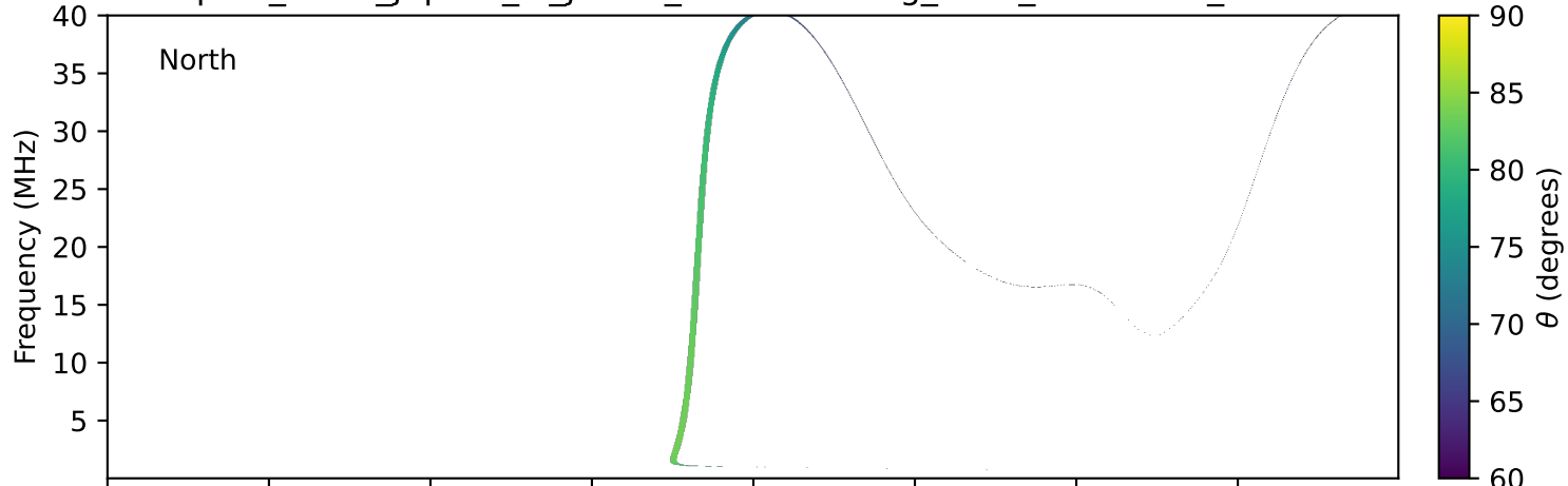
expres_earth_jupiter_io_jrm33_lossc-wid1deg_3kev_20131107_v11.cdf
