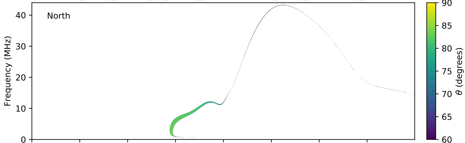
expres_earth_jupiter_io_jrm09_lossc-wid1deg_3kev_20131130_v01.cdf
