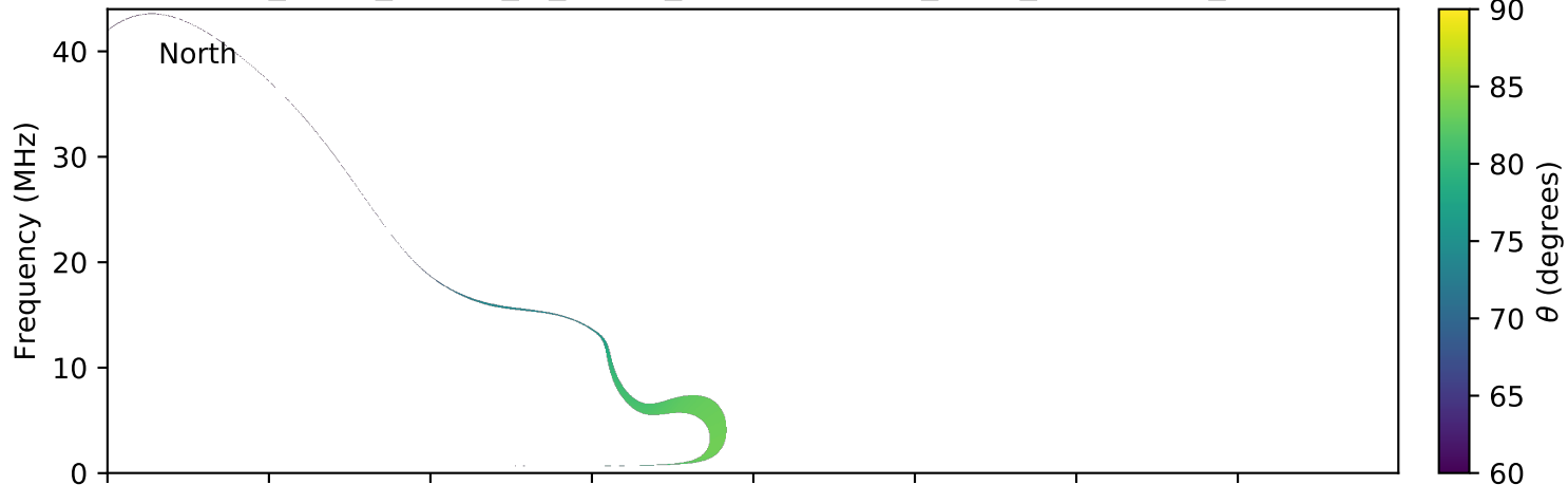
expres_earth_jupiter_io_jrm09_lossc-wid1deg_3kev_20131129_v01.cdf
