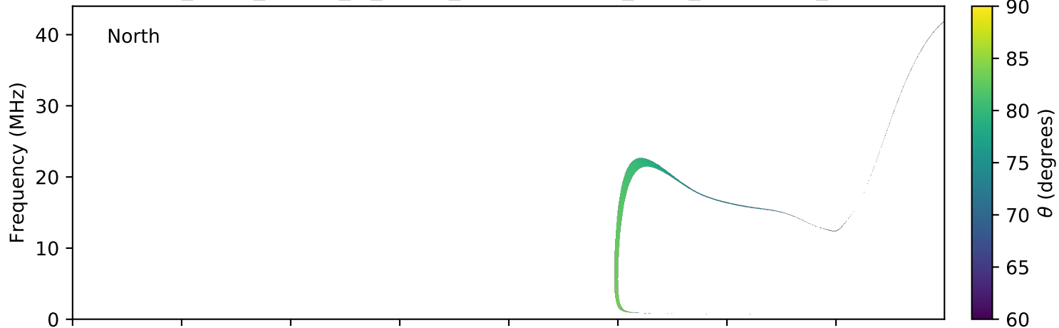
expres_earth_jupiter_io_jrm09_lossc-wid1deg_3kev_20131128_v01.cdf
