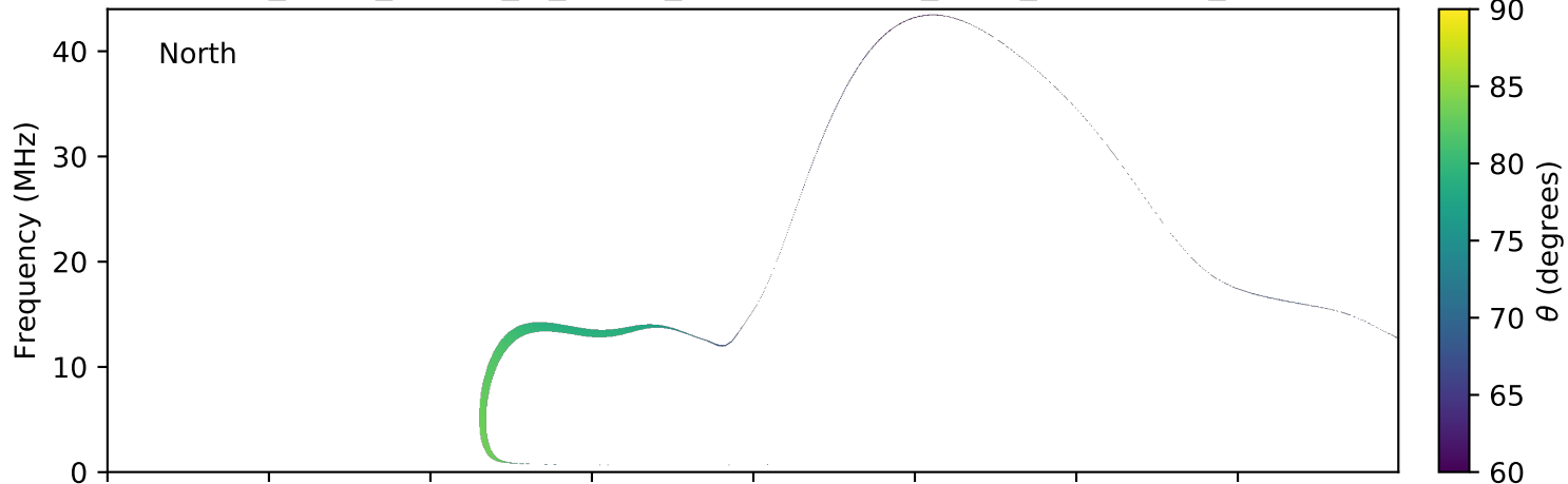
expres_earth_jupiter_io_jrm09_lossc-wid1deg_3kev_20131123_v01.cdf
