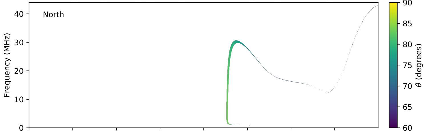
expres_earth_jupiter_io_jrm09_lossc-wid1deg_3kev_20131121_v01.cdf
