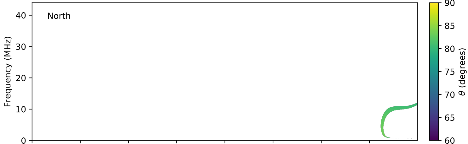
expres_earth_jupiter_io_jrm09_lossc-wid1deg_3kev_20131110_v01.cdf
