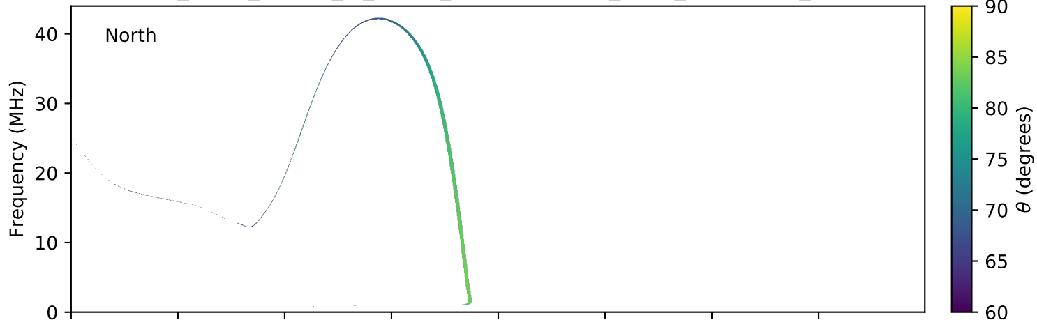
expres_earth_jupiter_io_jrm09_lossc-wid1deg_3kev_20131106_v01.cdf
