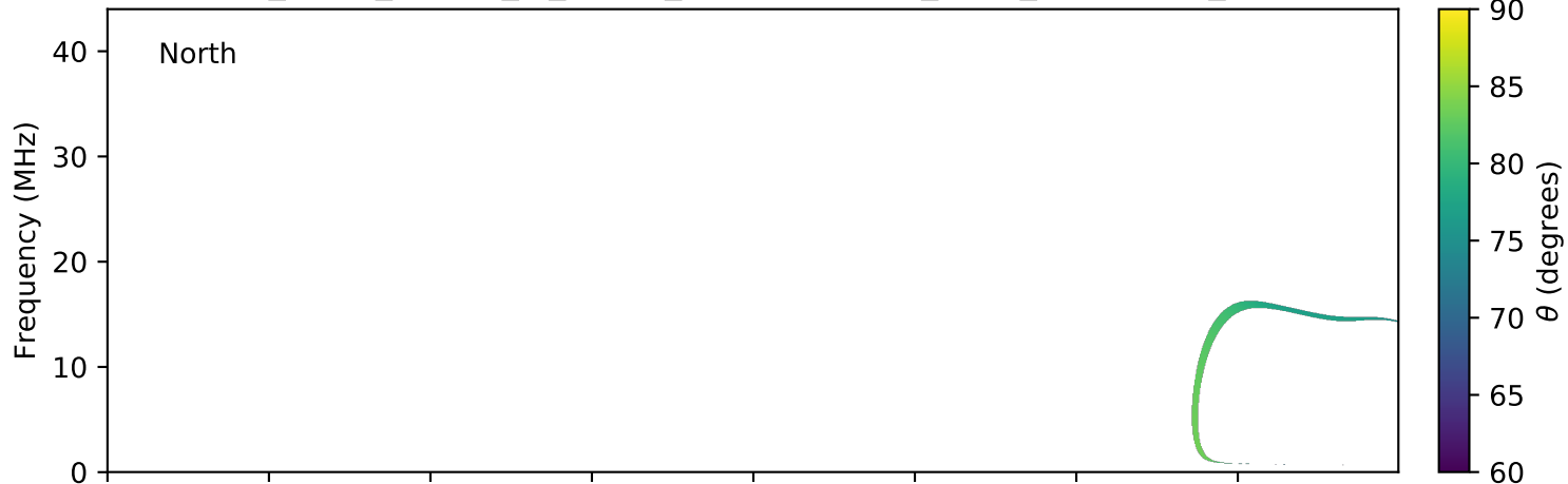
expres_earth_jupiter_io_jrm09_lossc-wid1deg_3kev_20131103_v01.cdf
