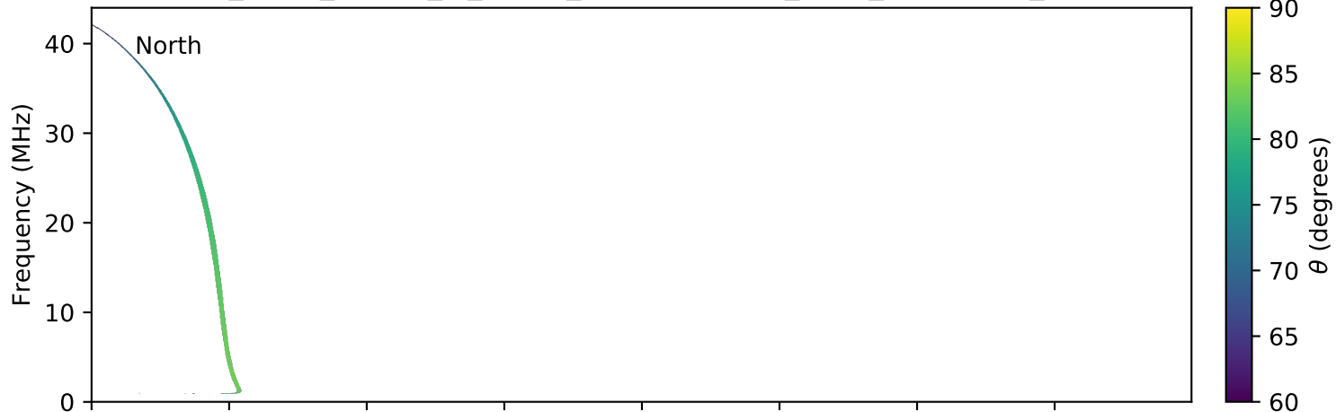
expres_earth_jupiter_io_jrm09_lossc-wid1deg_3kev_20131101_v01.cdf
