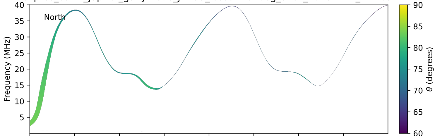
expres_earth_jupiter_ganymede_jrm33_lossc-wid1deg_3kev_20131114_v11.cdf
