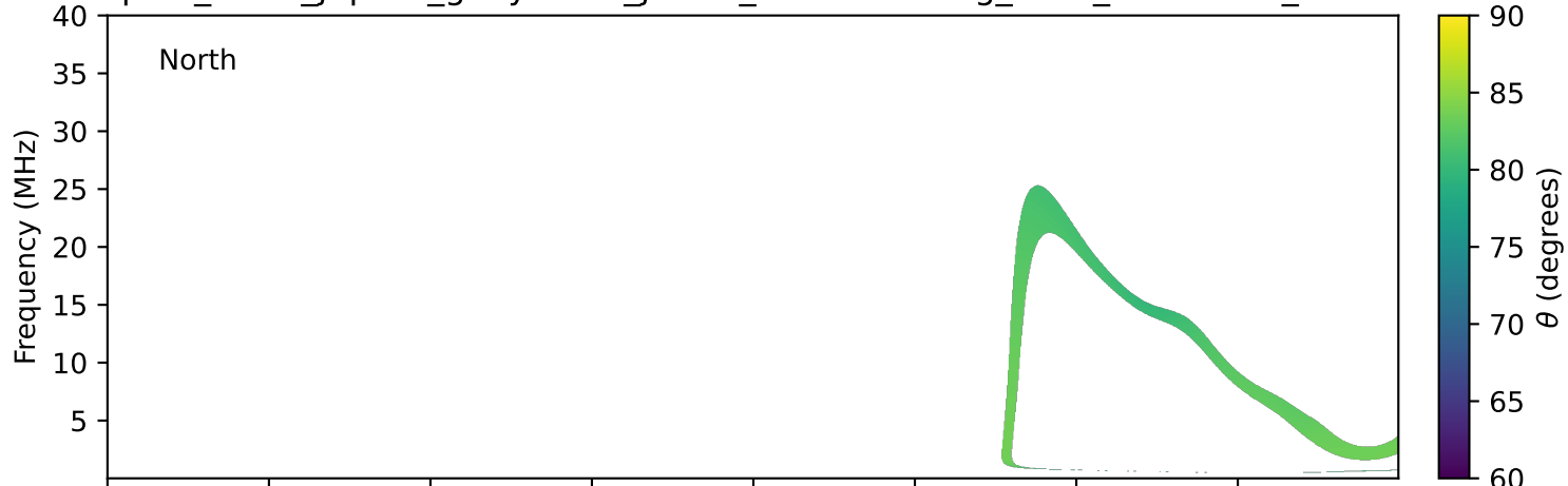
expres_earth_jupiter_ganymede_jrm33_lossc-wid1deg_3kev_20131113_v11.cdf
