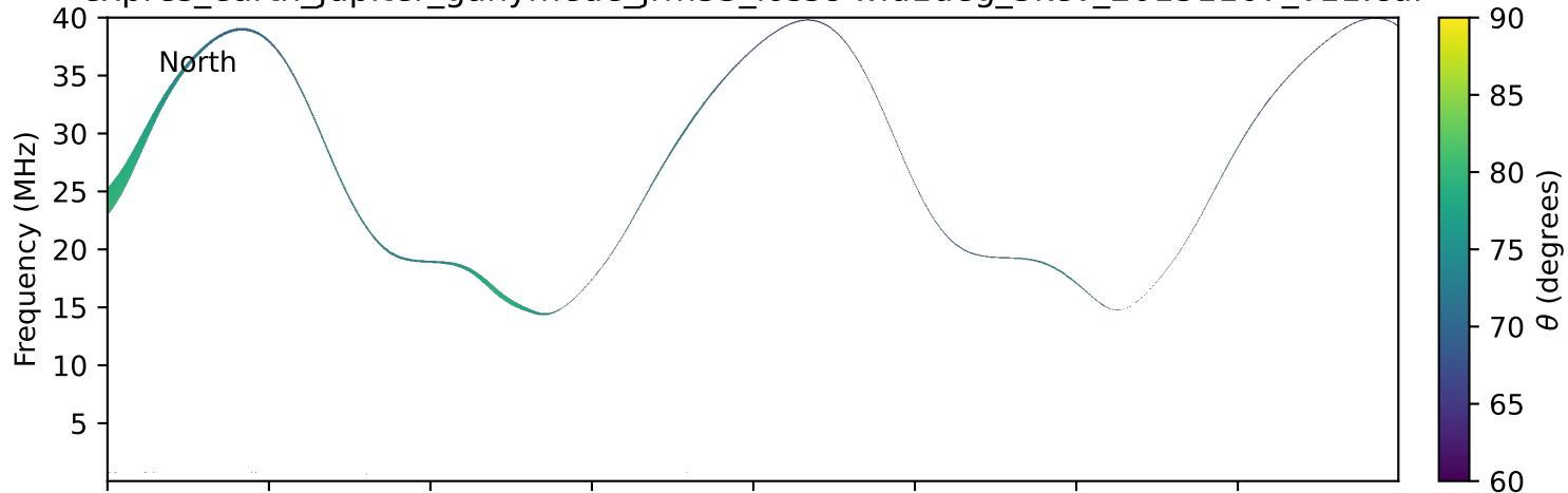
expres_earth_jupiter_ganymede_jrm33_lossc-wid1deg_3kev_20131107_v11.cdf
