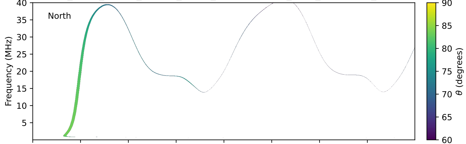
expres_earth_jupiter_europa_jrm33_lossc-wid1deg_3kev_20131116_v11.cdf
