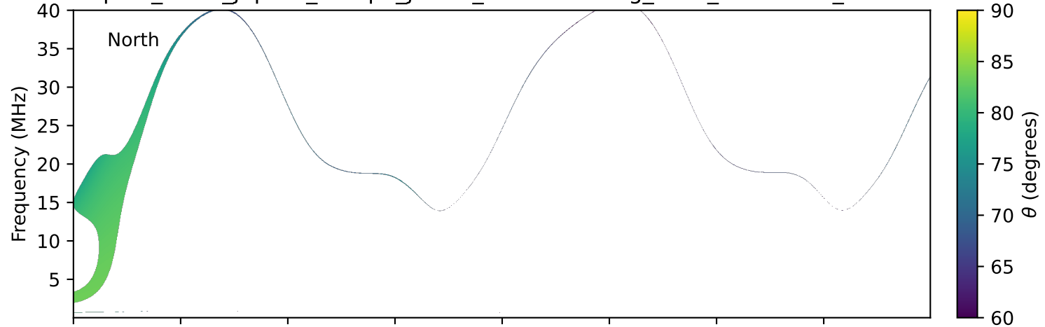
expres_earth_jupiter_europa_jrm33_lossc-wid1deg_3kev_20131109_v11.cdf
