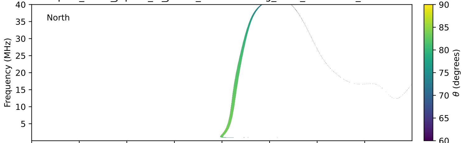
expres_earth_jupiter_io_jrm33_lossc-wid1deg_3kev_20130929_v11.cdf
