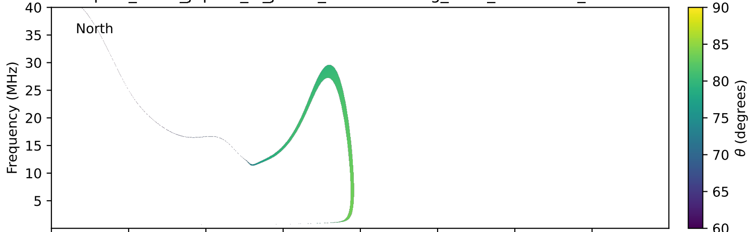
expres_earth_jupiter_io_jrm33_lossc-wid1deg_3kev_20130921_v11.cdf
