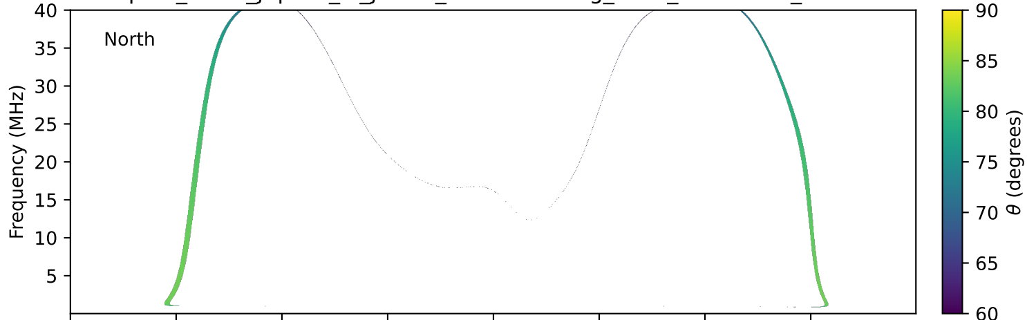
expres_earth_jupiter_io_jrm33_lossc-wid1deg_3kev_20130917_v11.cdf
