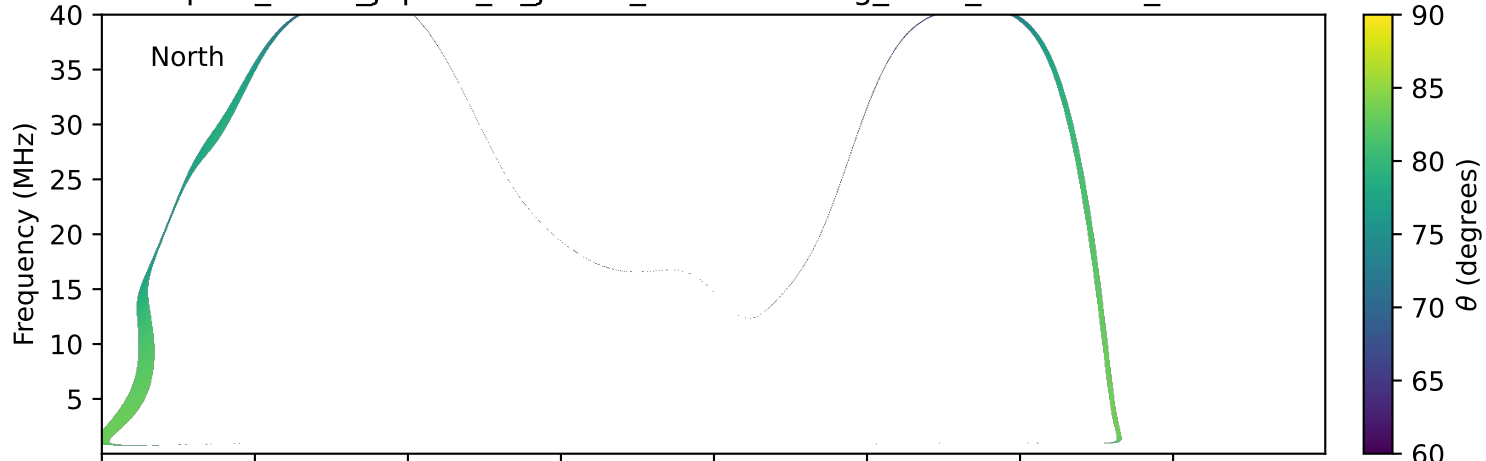
expres_earth_jupiter_io_jrm33_lossc-wid1deg_3kev_20130910_v11.cdf
