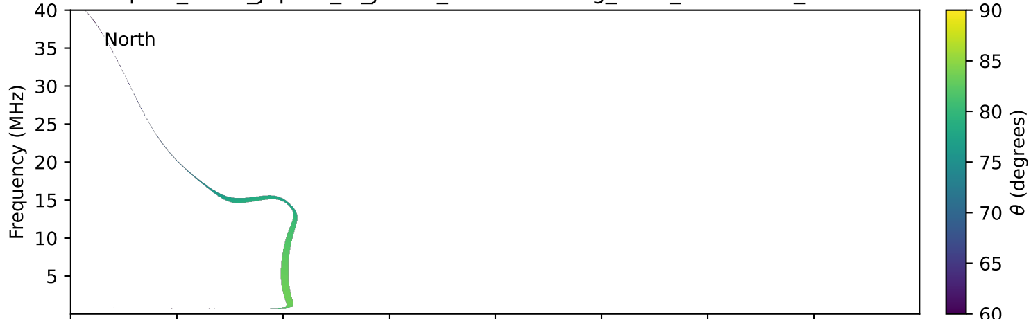
expres_earth_jupiter_io_jrm33_lossc-wid1deg_3kev_20130907_v11.cdf
