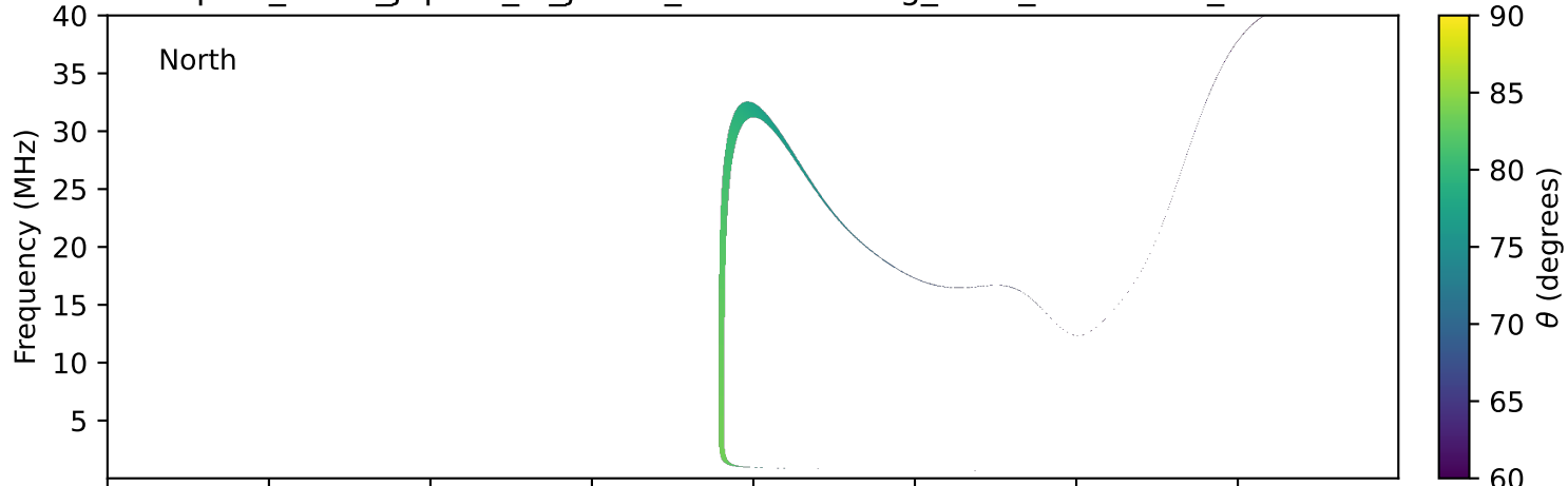
expres_earth_jupiter_io_jrm33_lossc-wid1deg_3kev_20130906_v11.cdf
